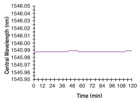
The temperature stabilization circuit ensures low central wavelength drift.
