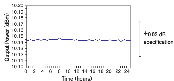
The source's excellent power stability output is ideal for long-term monitoring.
